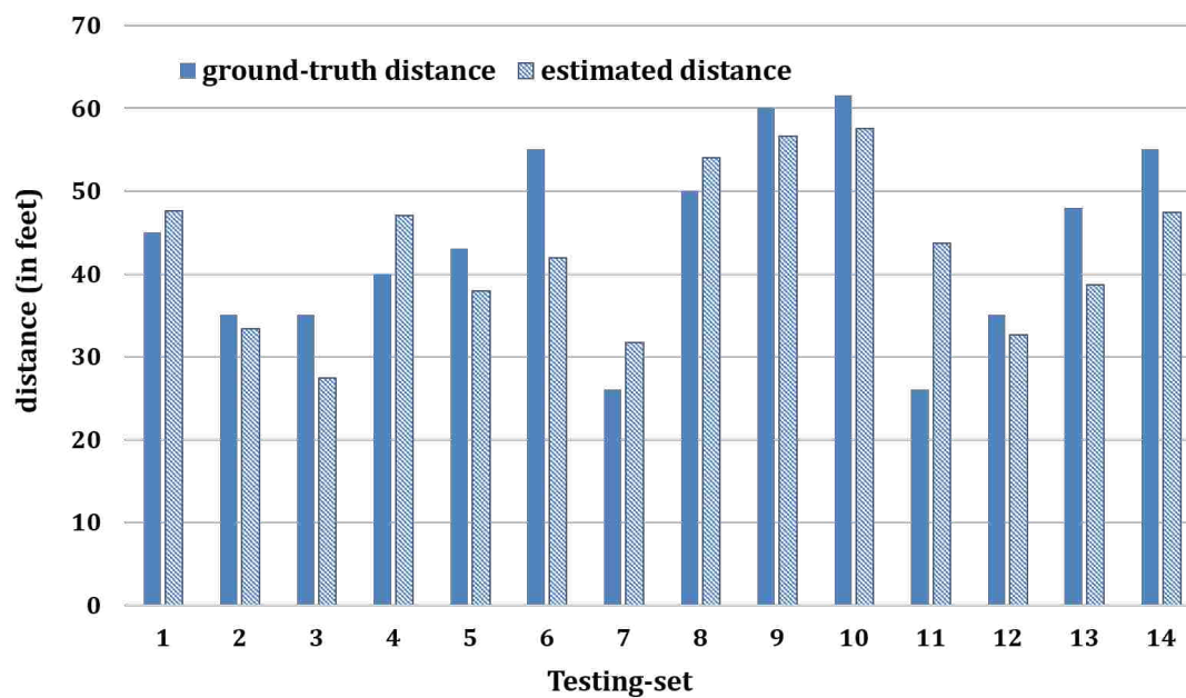
Figure 7.4. Distance estimation
