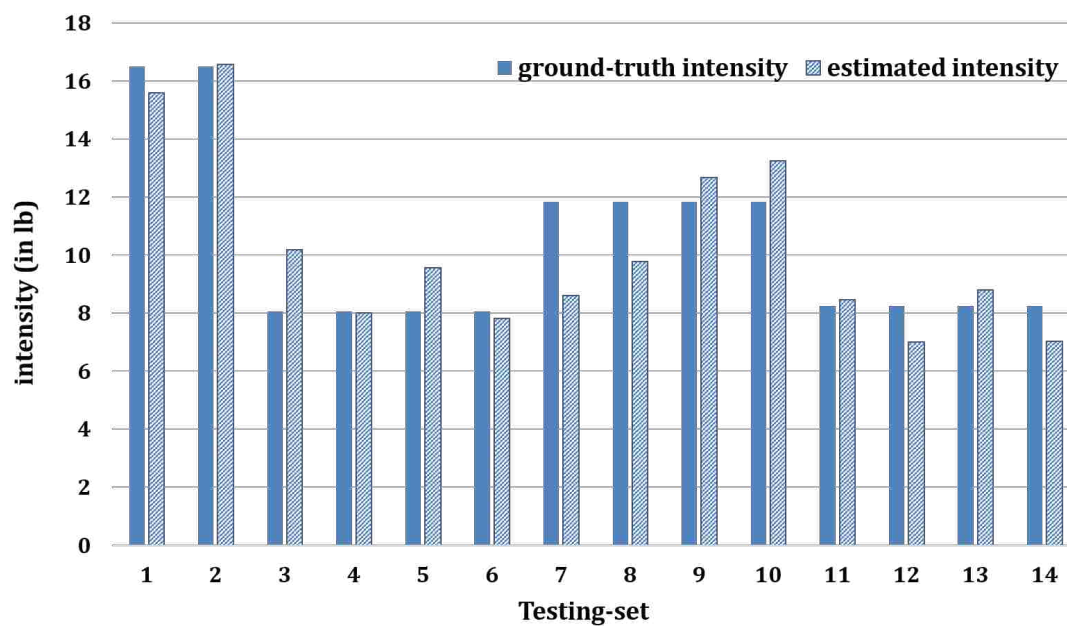
Figure 7.5. Intensity estimation
